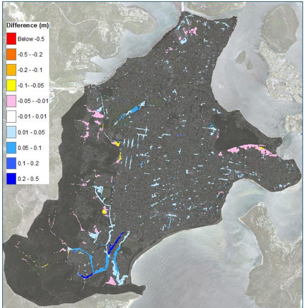
Figure 8.15 Difference in flood depth of 1% AEP 6hrs (ARR 1987 rainfall minus Baseline)
