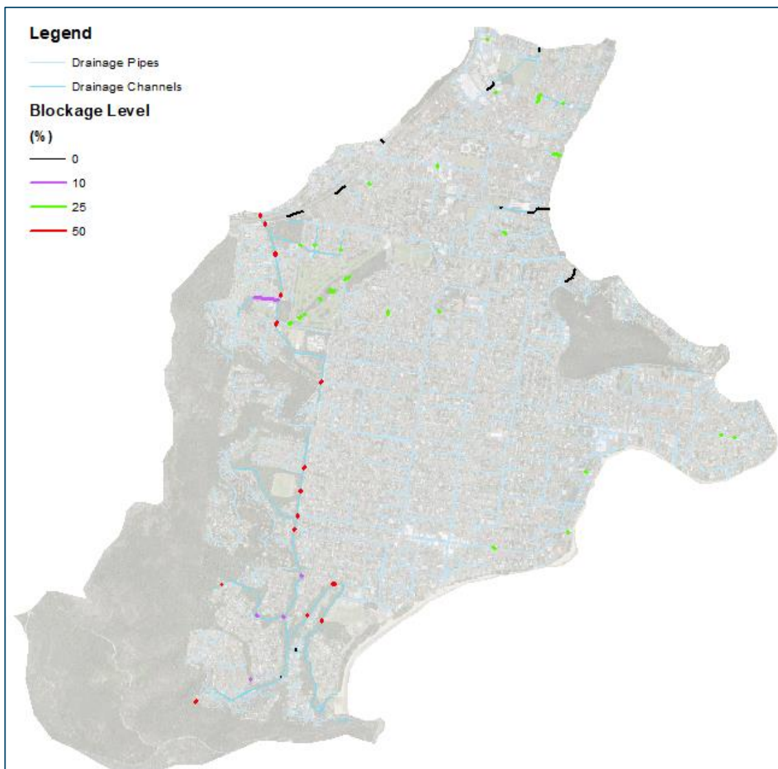
Figure 8.10 Inlet drainage blockage levels assumed for culvert structures
