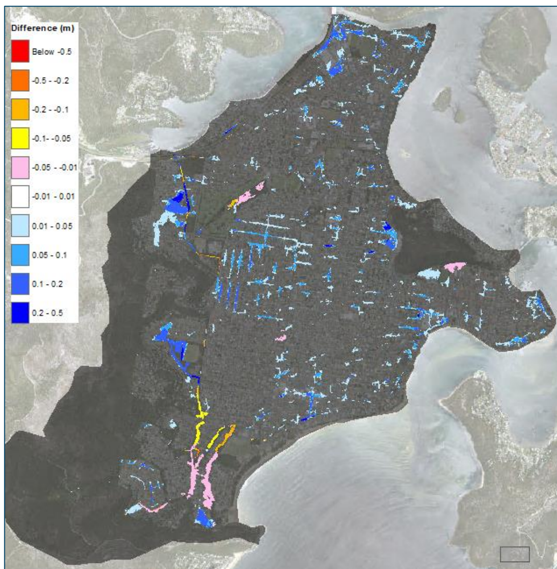
Figure 8.11 Difference in flood depth (Blockage minus Baseline)
