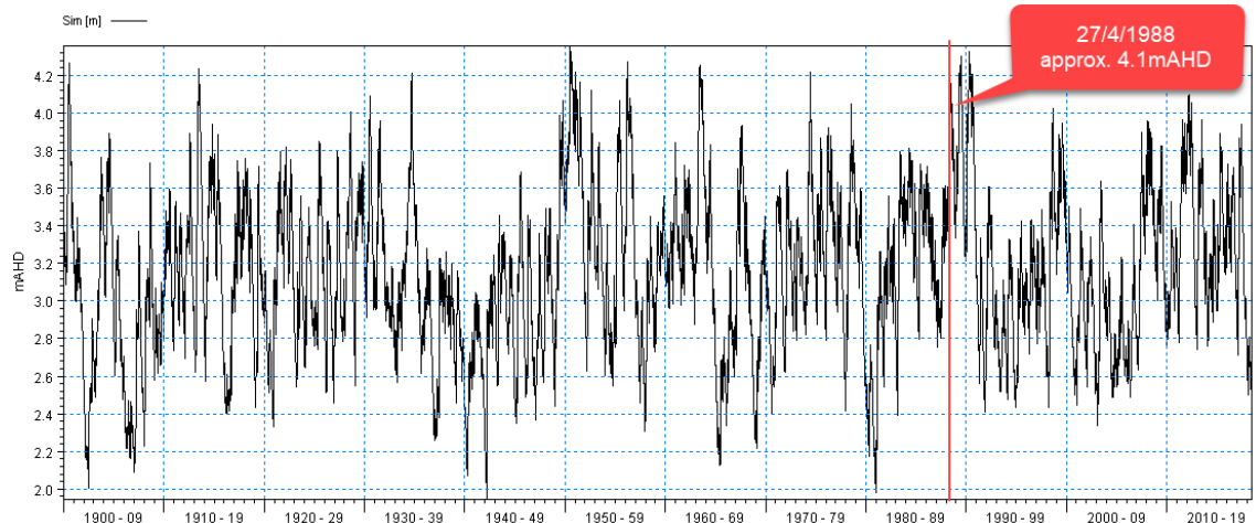
Figure 6.4 Simulated groundwater level at WW43 (near the intersection of Ryans Road and Shepard Street)
