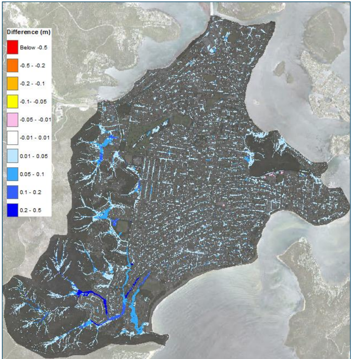
Figure 8.16 Difference in flood depth of 5% AEP 2hrs (ARR 1987 rainfall minus Baseline)
