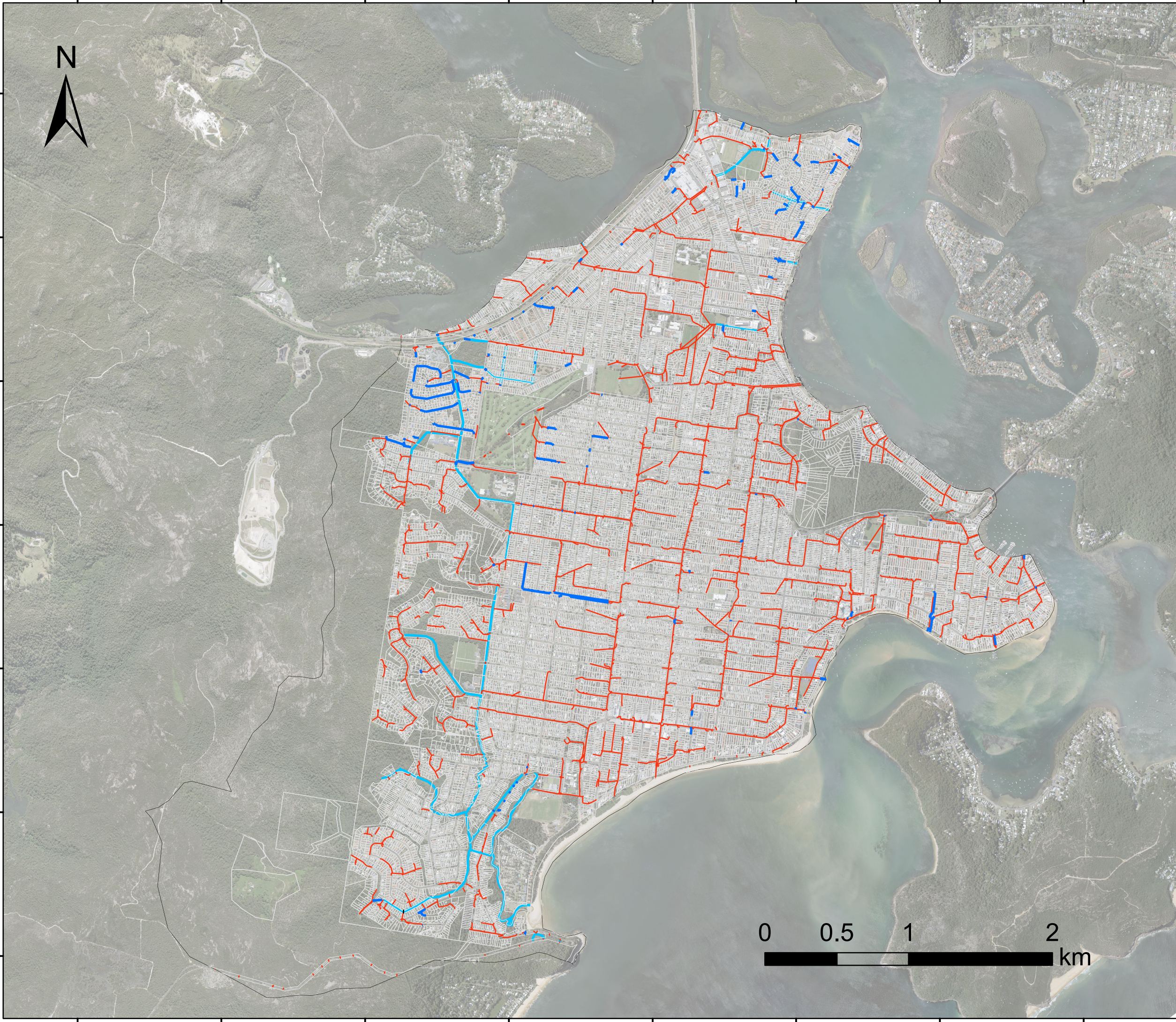
FIGURE C.2 Drainage Evaluation Invert Level Information
