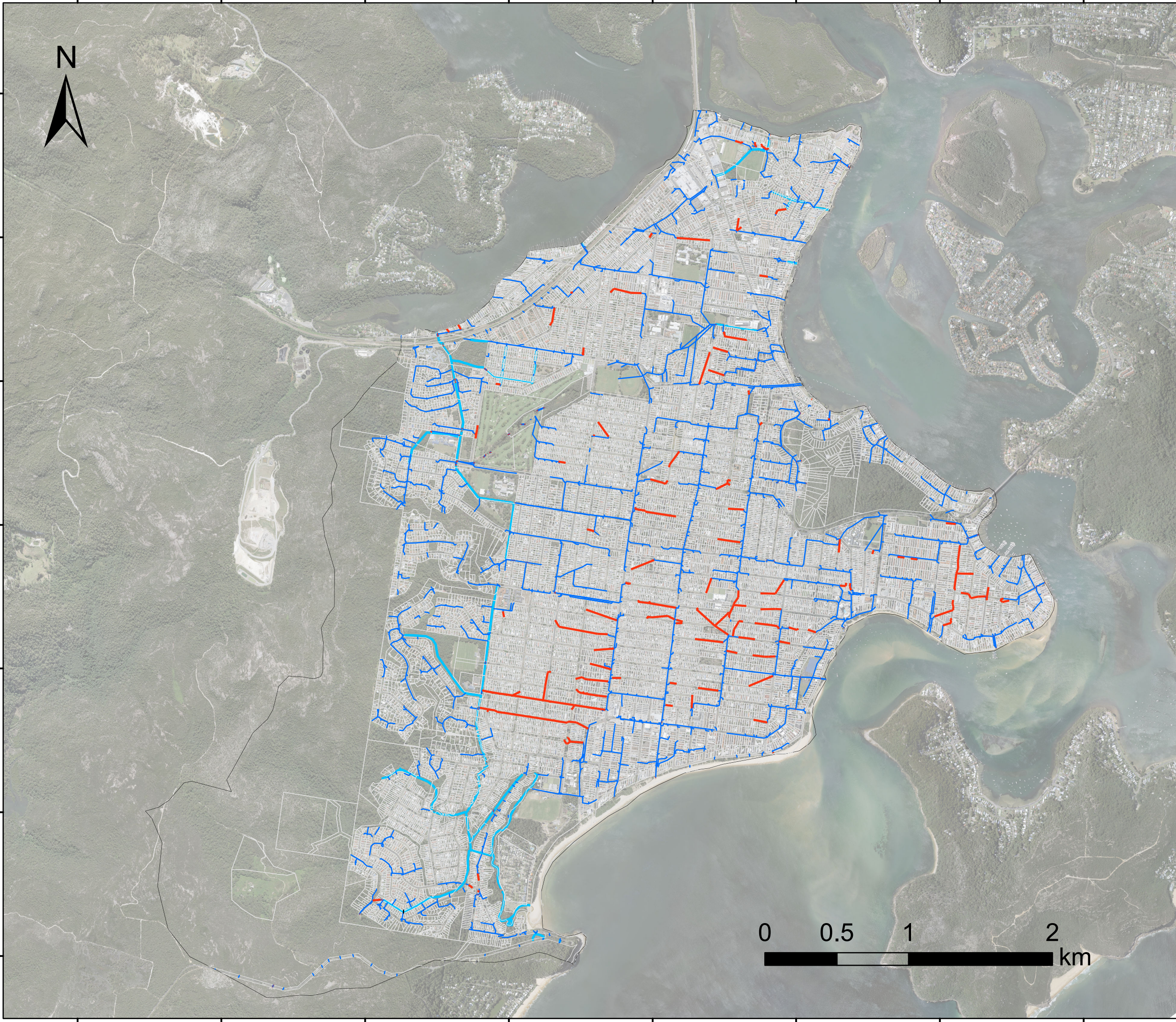
FIGURE C.1 Drainage Evaluation Diameter Information
